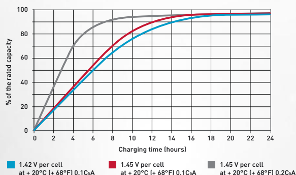
Available capacity after constant voltage charge Available charge current 0.1C 5 A for M type cell
