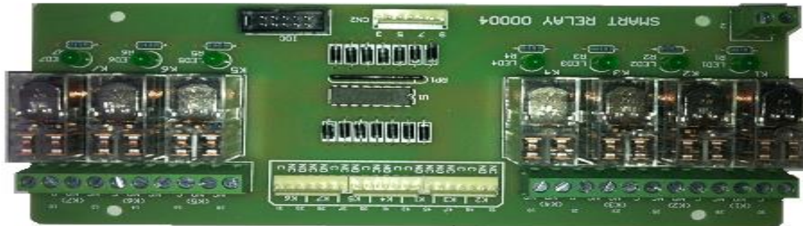
Smart Relay Interface Card
